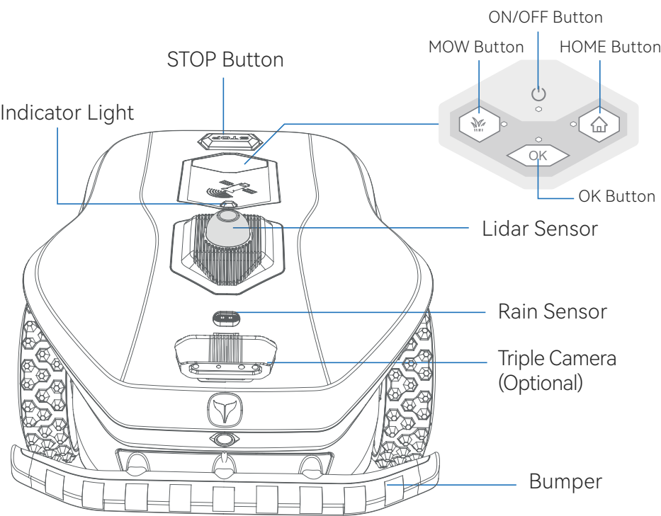
Top View
